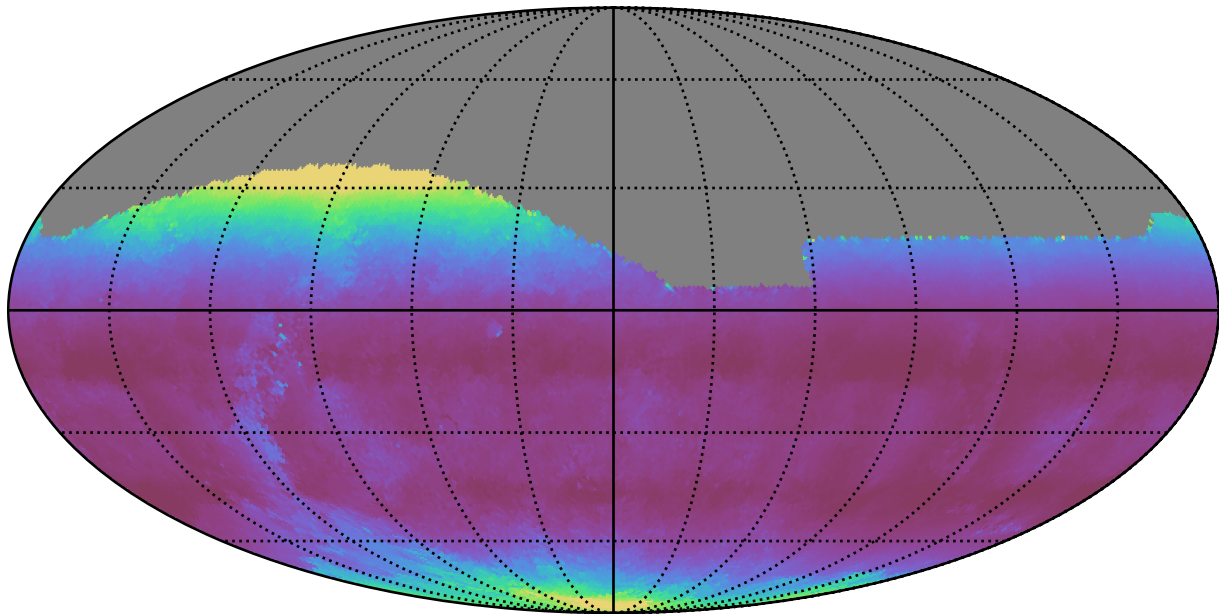
weather_cloudso36v3.4_10yrs All sky g band: Median airmass
