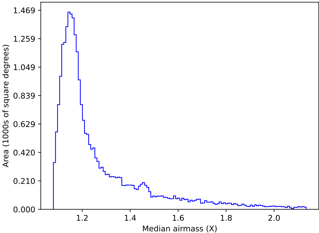
weather_cloudso36v3.4_10yrs All sky g band: Median airmass
