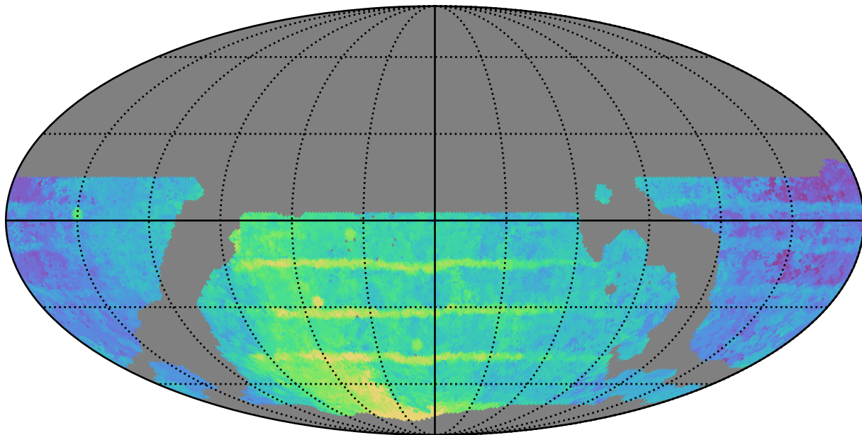
weather_cloudso36v3.4_10yrs WFD z band: Median Season Length
