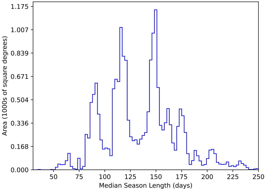
weather_cloudso36v3.4_10yrs WFD y band: Median Season Length
