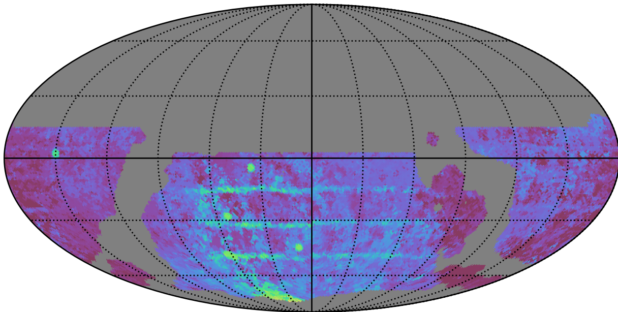
weather_cloudso36v3.4_10yrs WFD u band: Median Season Length
