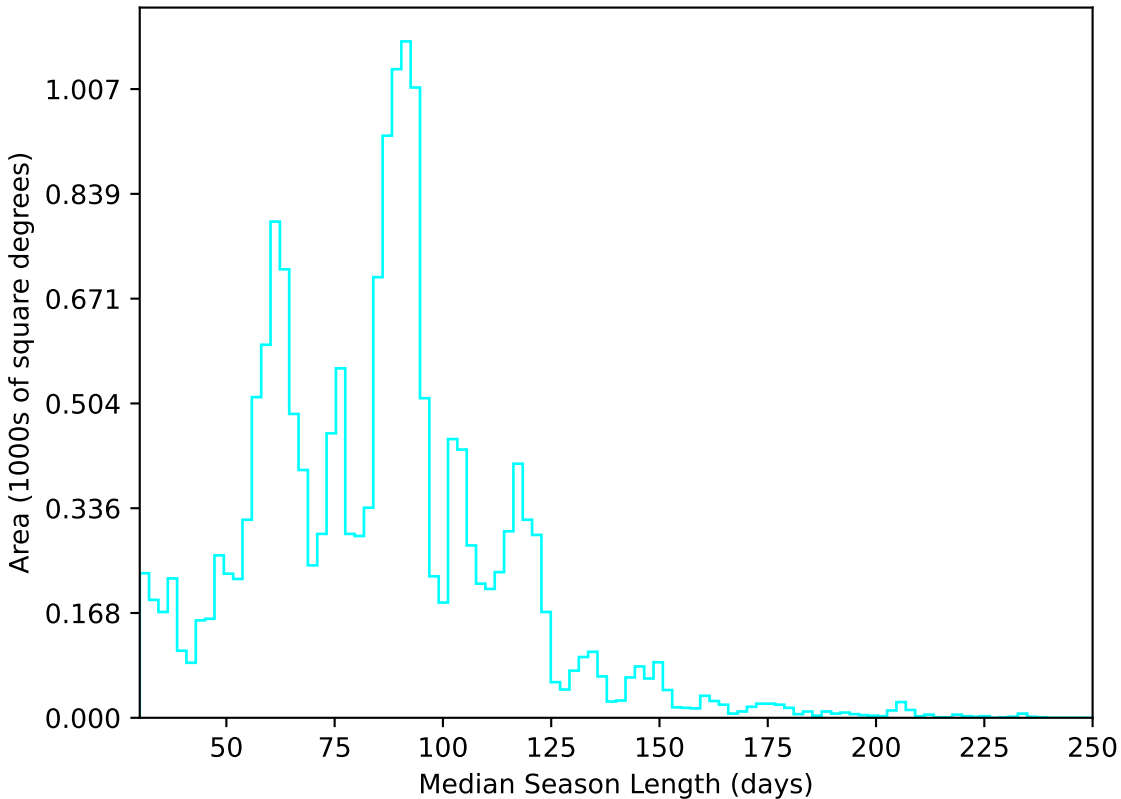
weather_cloudso36v3.4_10yrs WFD u band: Median Season Length
