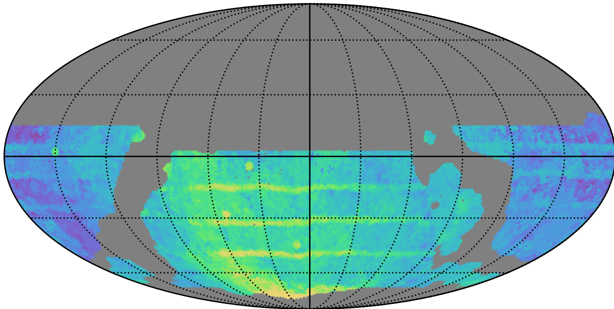
weather_cloudso36v3.4_10yrs WFD r band: Median Season Length
