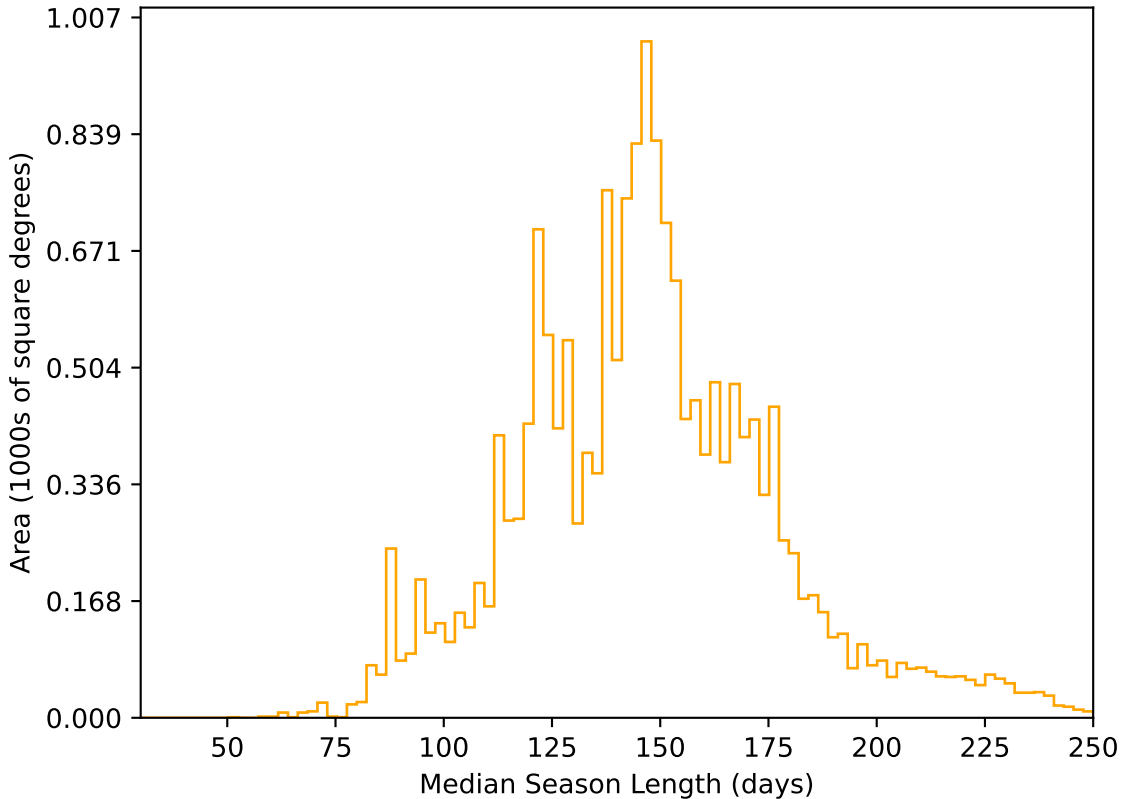
weather_cloudso36v3.4_10yrs WFD r band: Median Season Length
