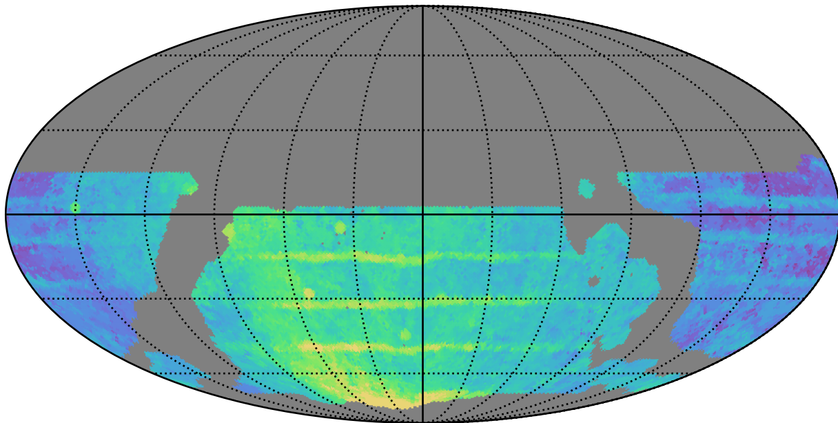
weather_cloudso36v3.4_10yrs WFD i band: Median Season Length
