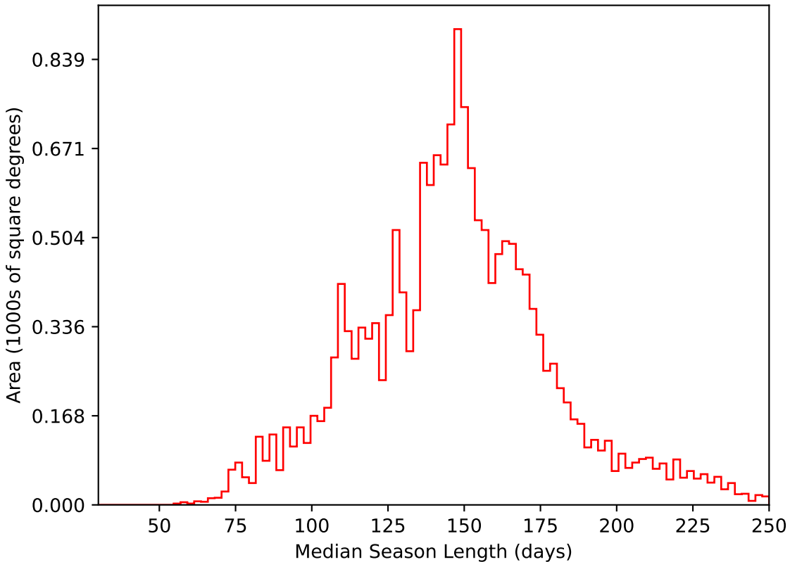
weather_cloudso36v3.4_10yrs WFD i band: Median Season Length
