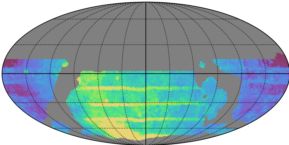
weather_cloudso36v3.4_10yrs WFD all bands: Median Season Length
