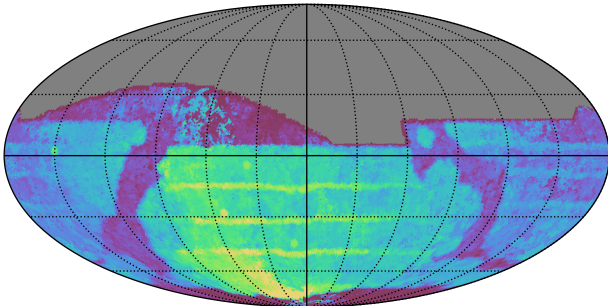
weather_cloudso36v3.4_10yrs All sky z band: Median Season Length
