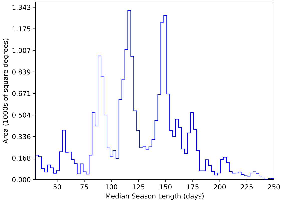
weather_cloudso36v3.4_10yrs All sky y band: Median Season Length
