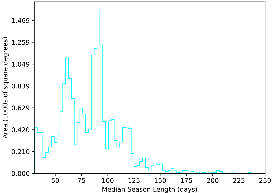
weather_cloudso36v3.4_10yrs All sky u band: Median Season Length
