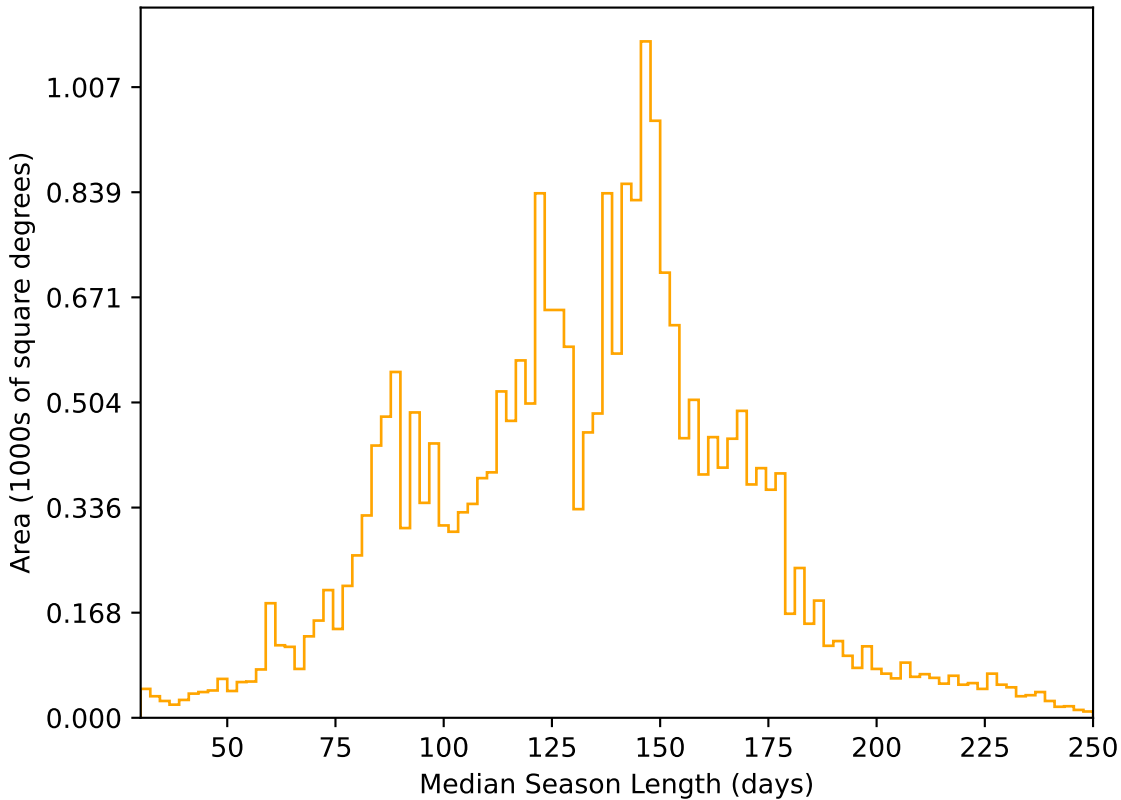
weather_cloudso36v3.4_10yrs All sky r band: Median Season Length
