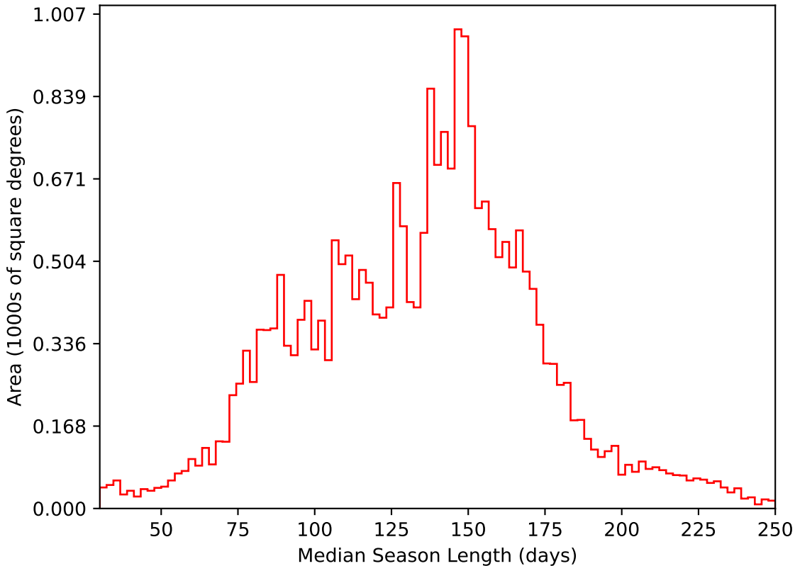
weather_cloudso36v3.4_10yrs All sky i band: Median Season Length
