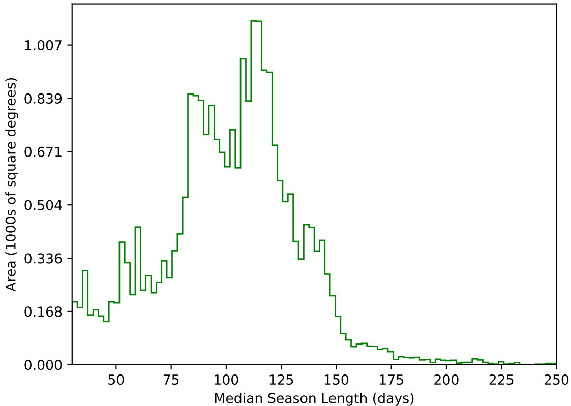
weather_cloudso36v3.4_10yrs All sky g band: Median Season Length
