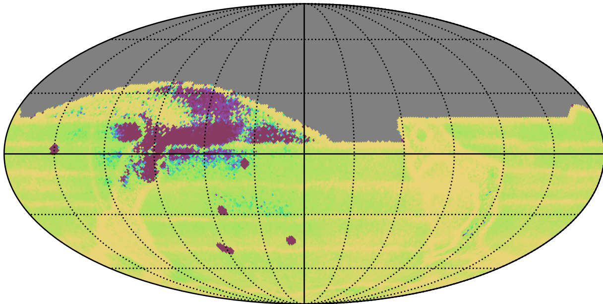
weather_cloudso36v3.4_10yrs All sky: Median Intra-Night Gap
