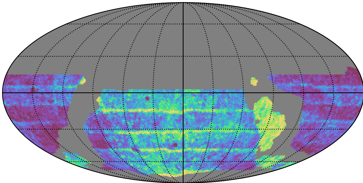
weather_cloudso36v3.4_10yrs WFD z band: Median Inter-Night Gap
