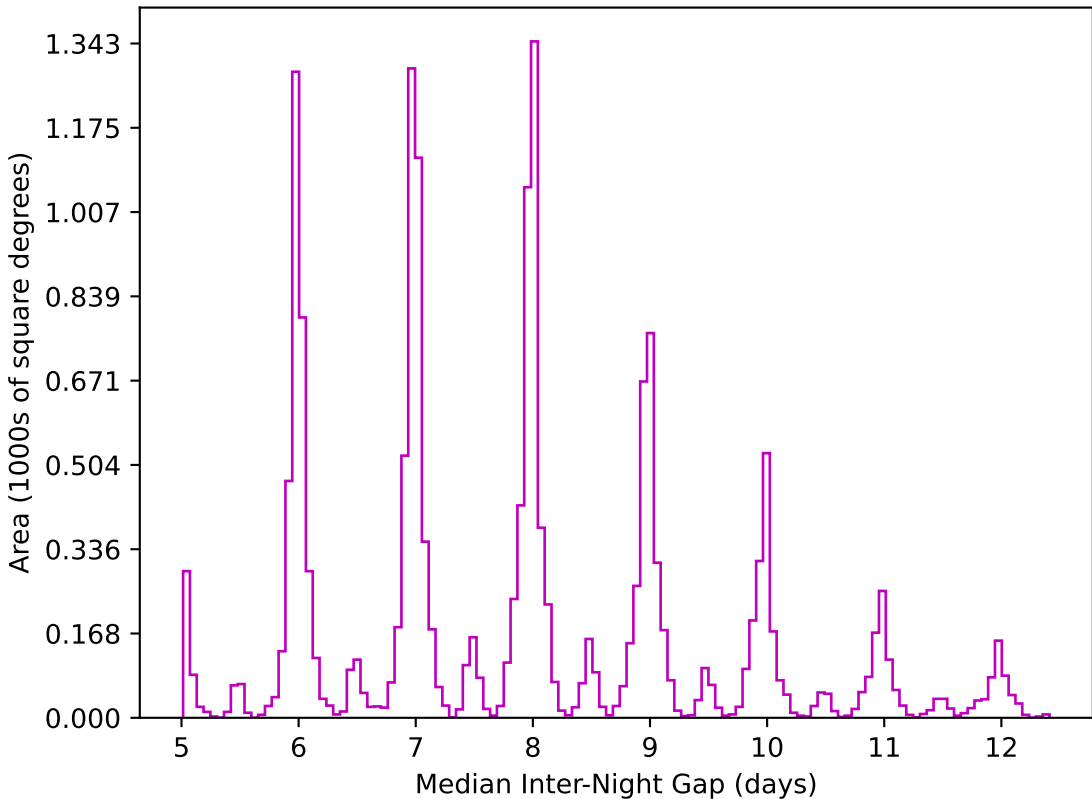
weather_cloudso36v3.4_10yrs WFD z band: Median Inter-Night Gap
