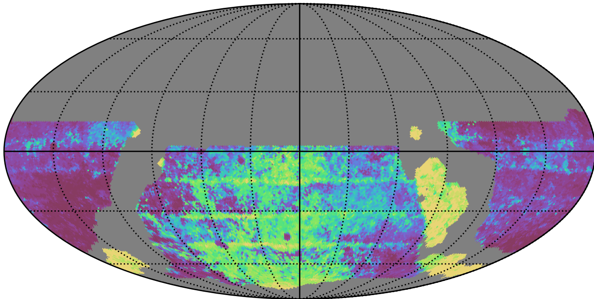
weather_cloudso36v3.4_10yrs WFD y band: Median Inter-Night Gap
