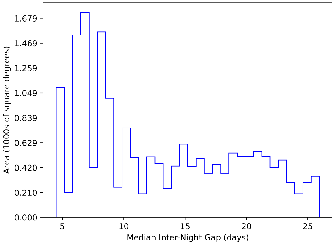
weather_cloudso36v3.4_10yrs WFD y band: Median Inter-Night Gap
