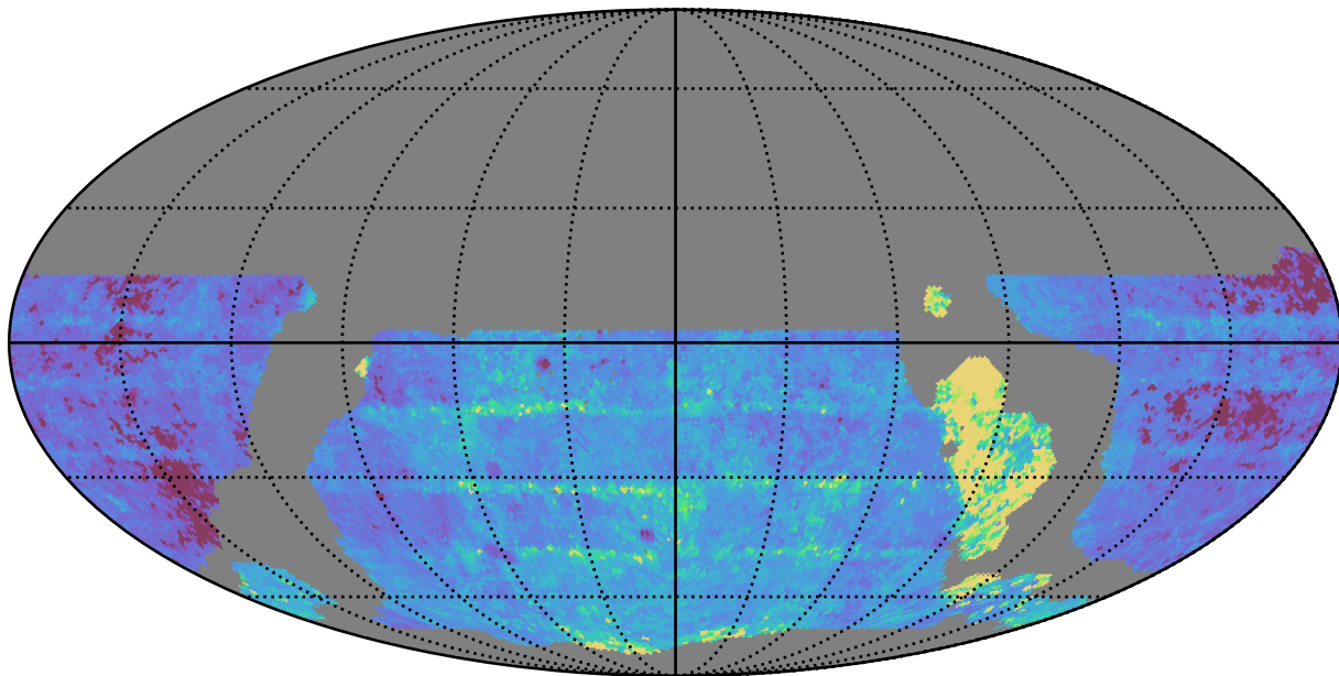
weather_cloudso36v3.4_10yrs WFD u band: Median Inter-Night Gap
