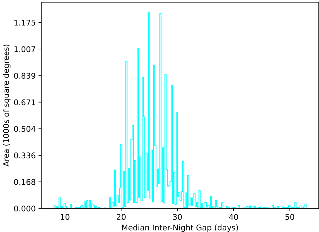
weather_cloudso36v3.4_10yrs WFD u band: Median Inter-Night Gap
