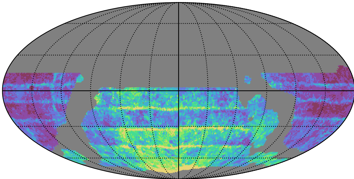
weather_cloudso36v3.4_10yrs WFD r band: Median Inter-Night Gap
