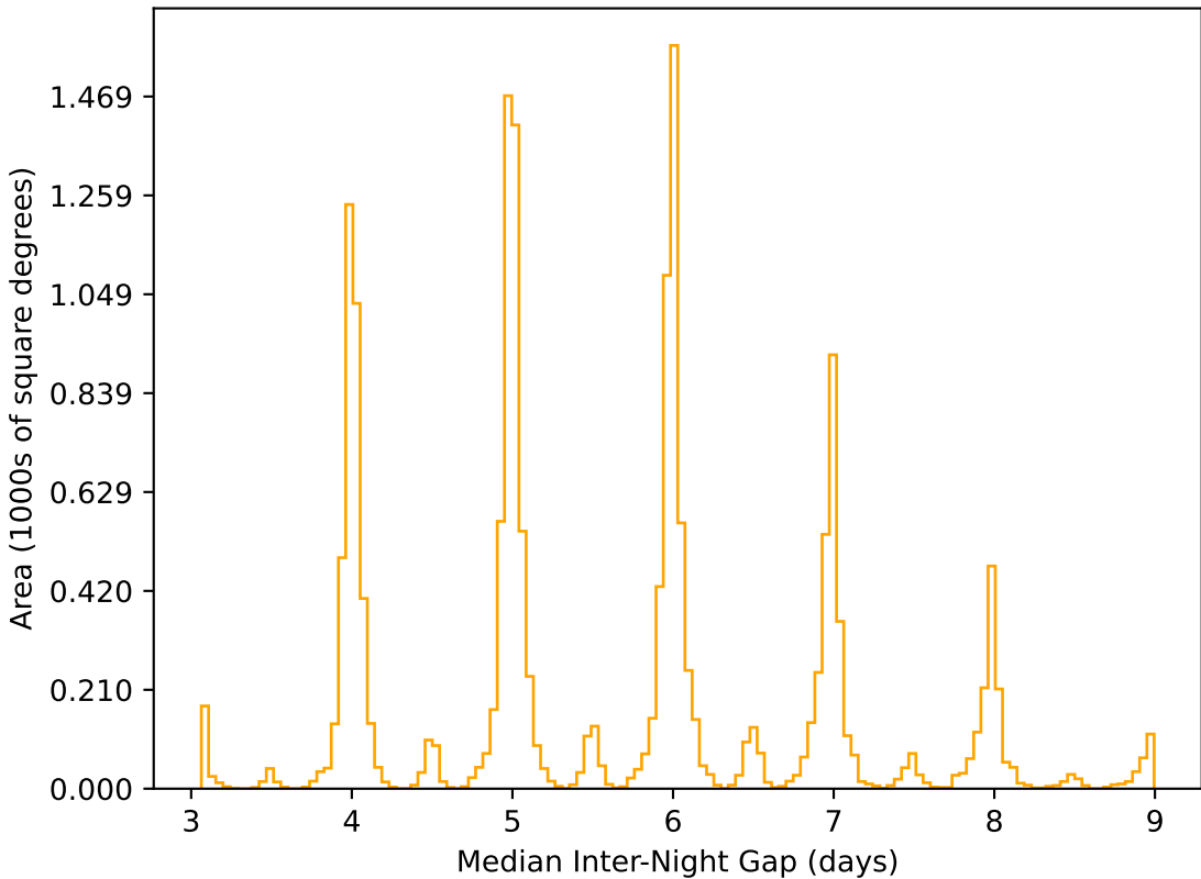
weather_cloudso36v3.4_10yrs WFD r band: Median Inter-Night Gap
