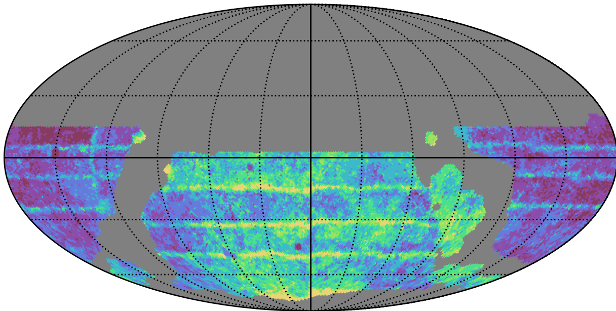
weather_cloudso36v3.4_10yrs WFD i band: Median Inter-Night Gap
