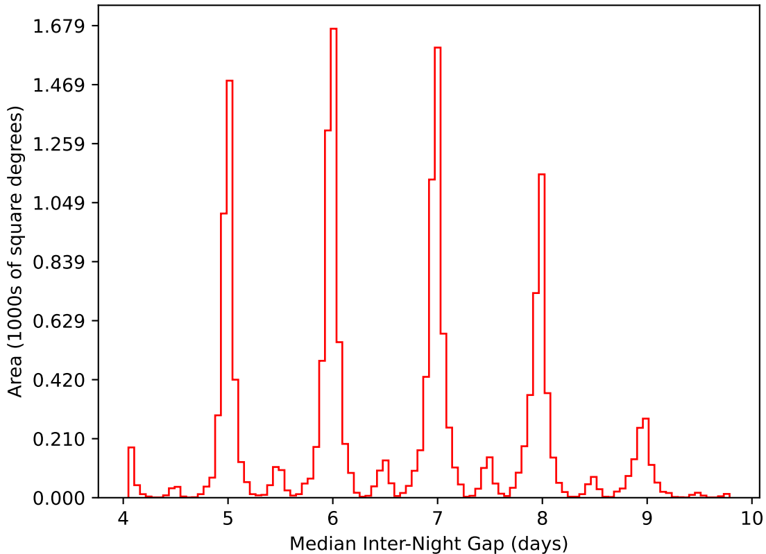
weather_cloudso36v3.4_10yrs WFD i band: Median Inter-Night Gap
