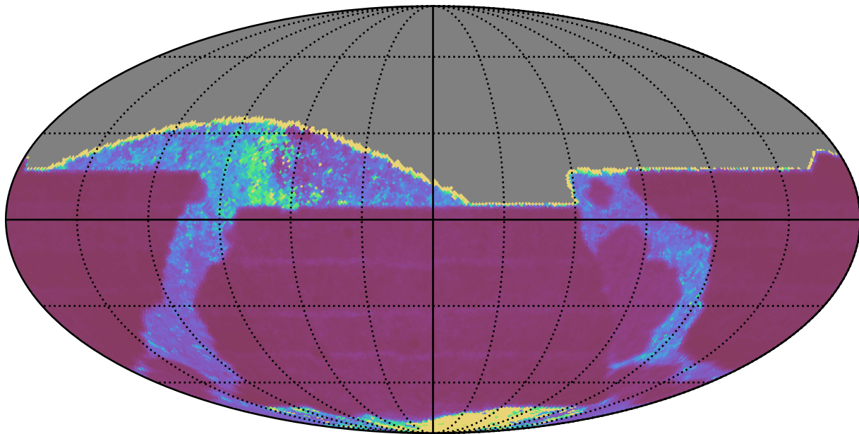
weather_cloudso36v3.4_10yrs All sky z band: Median Inter-Night Gap
