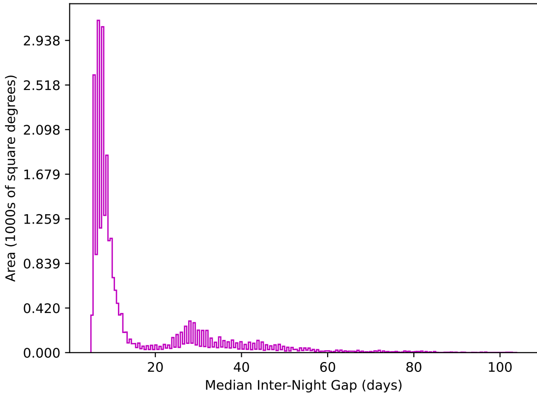
weather_cloudso36v3.4_10yrs All sky z band: Median Inter-Night Gap
