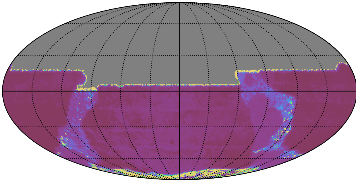
weather_cloudso36v3.4_10yrs All sky y band: Median Inter-Night Gap
