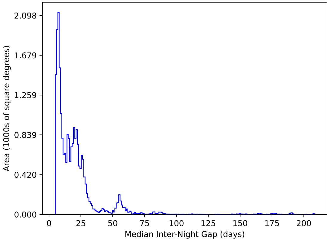
weather_cloudso36v3.4_10yrs All sky y band: Median Inter-Night Gap
