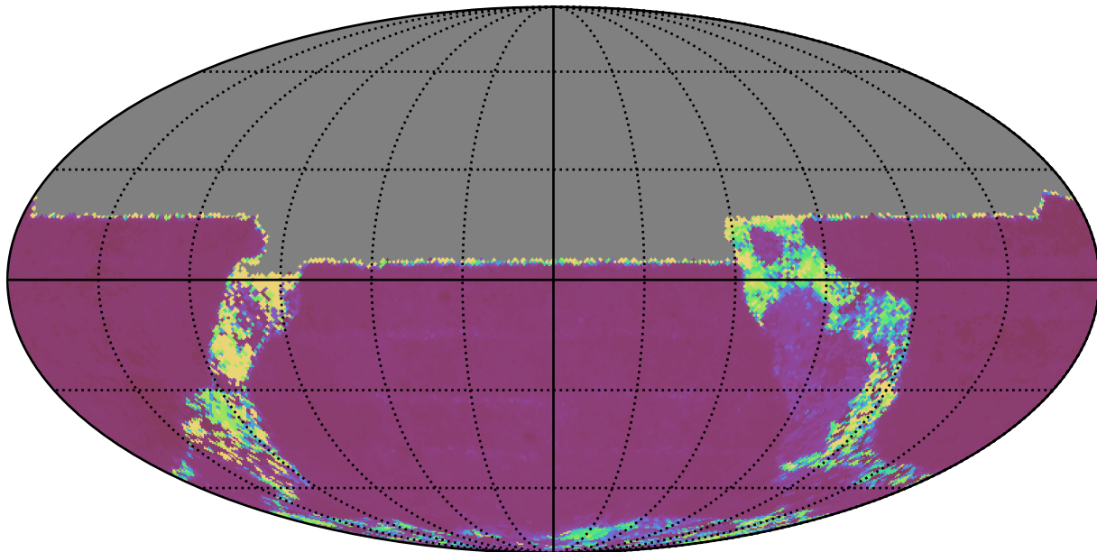
weather_cloudso36v3.4_10yrs All sky u band: Median Inter-Night Gap
