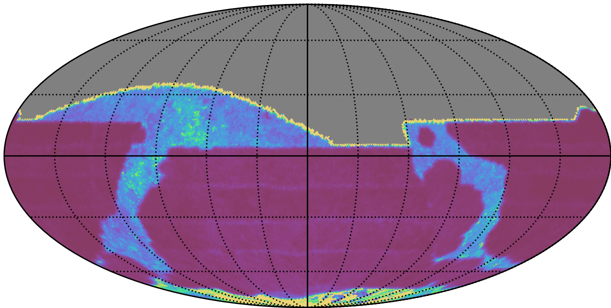
weather_cloudso36v3.4_10yrs All sky r band: Median Inter-Night Gap
