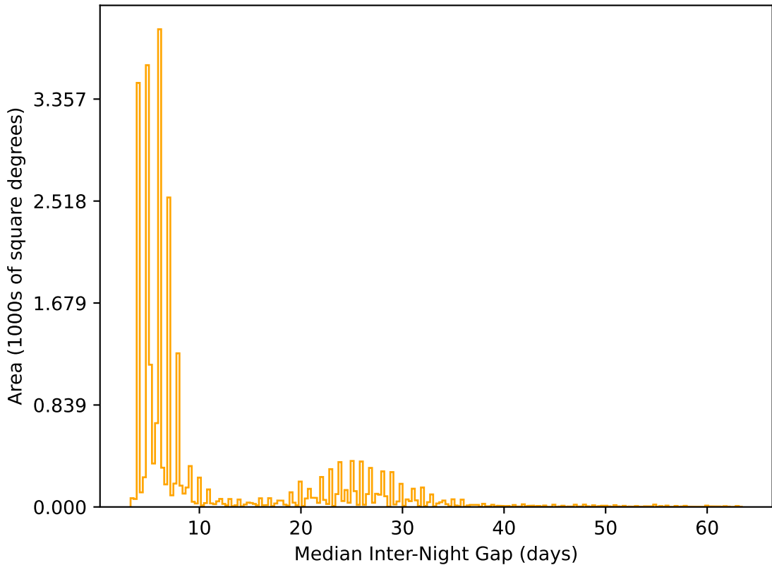
weather_cloudso36v3.4_10yrs All sky r band: Median Inter-Night Gap
