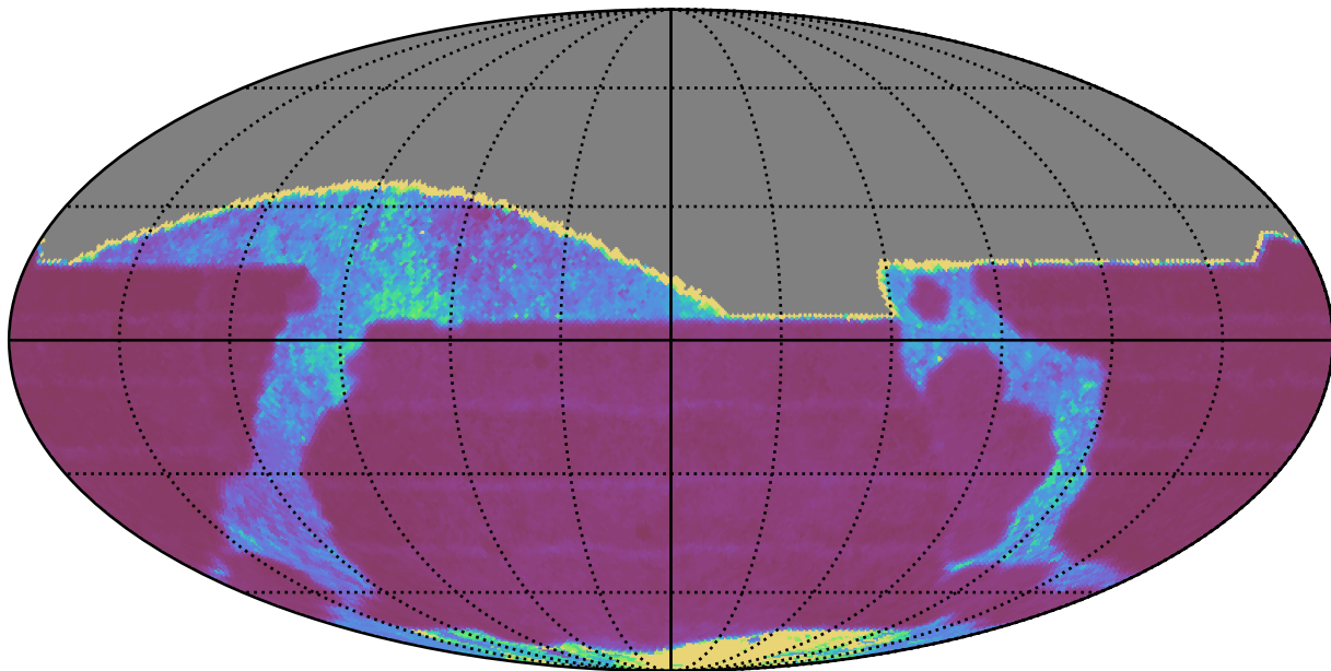
weather_cloudso36v3.4_10yrs All sky i band: Median Inter-Night Gap
