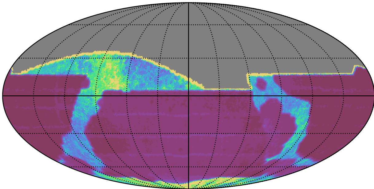
weather_cloudso36v3.4_10yrs All sky all bands: Median Inter-Night Gap
