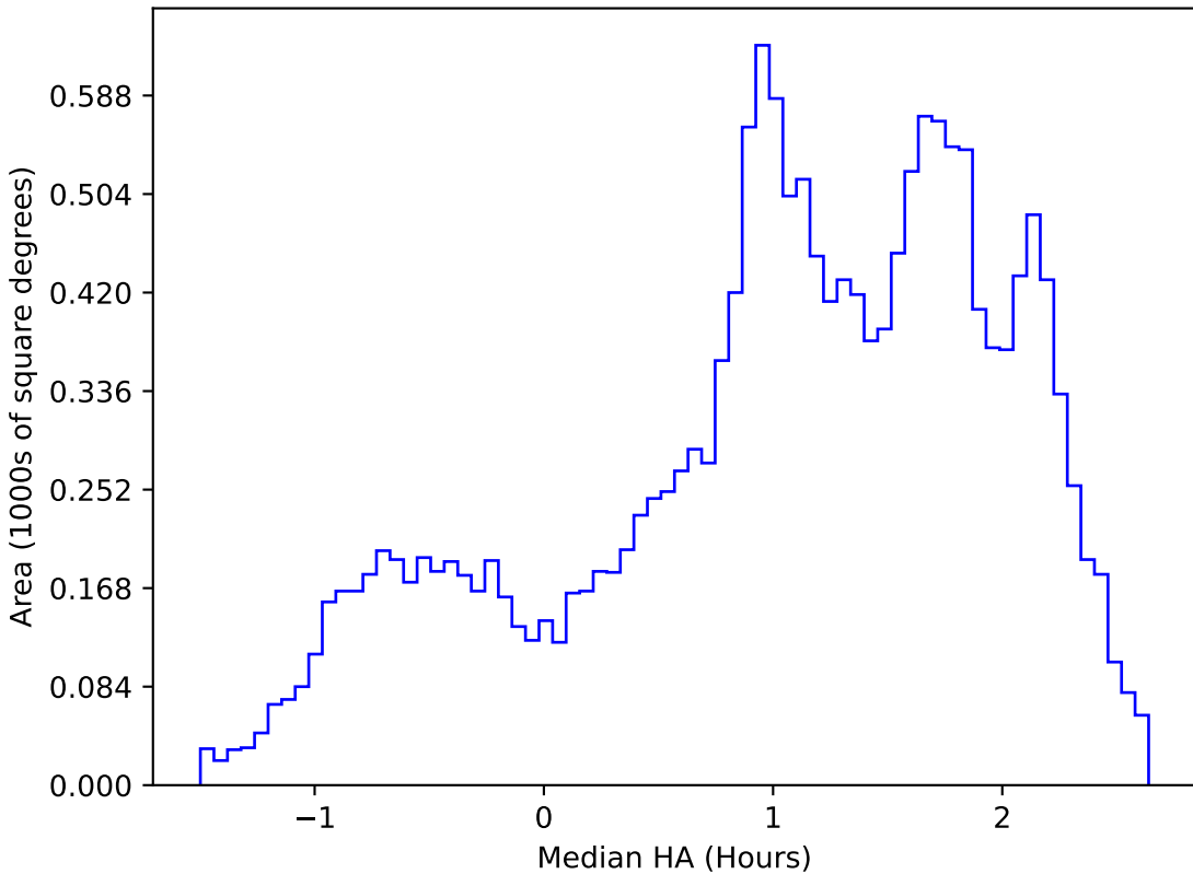
weather_cloudso36v3.4_10yrs WFD z band: Median HA
