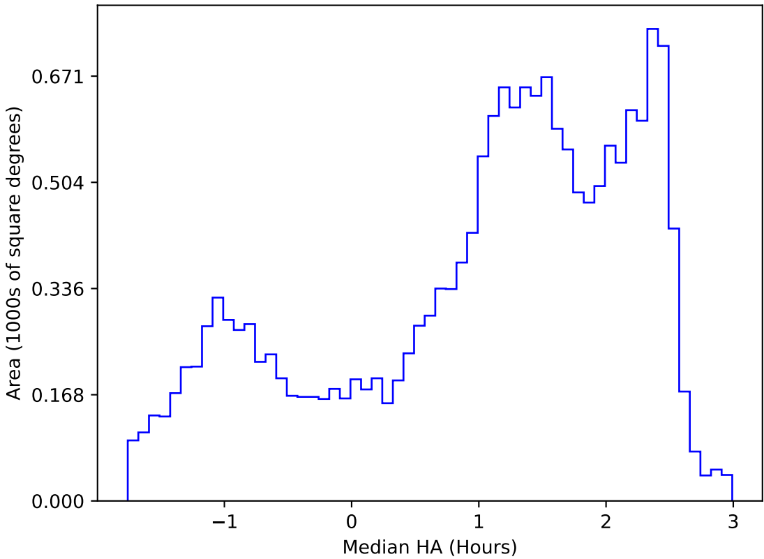
weather_cloudso36v3.4_10yrs WFD y band: Median HA
