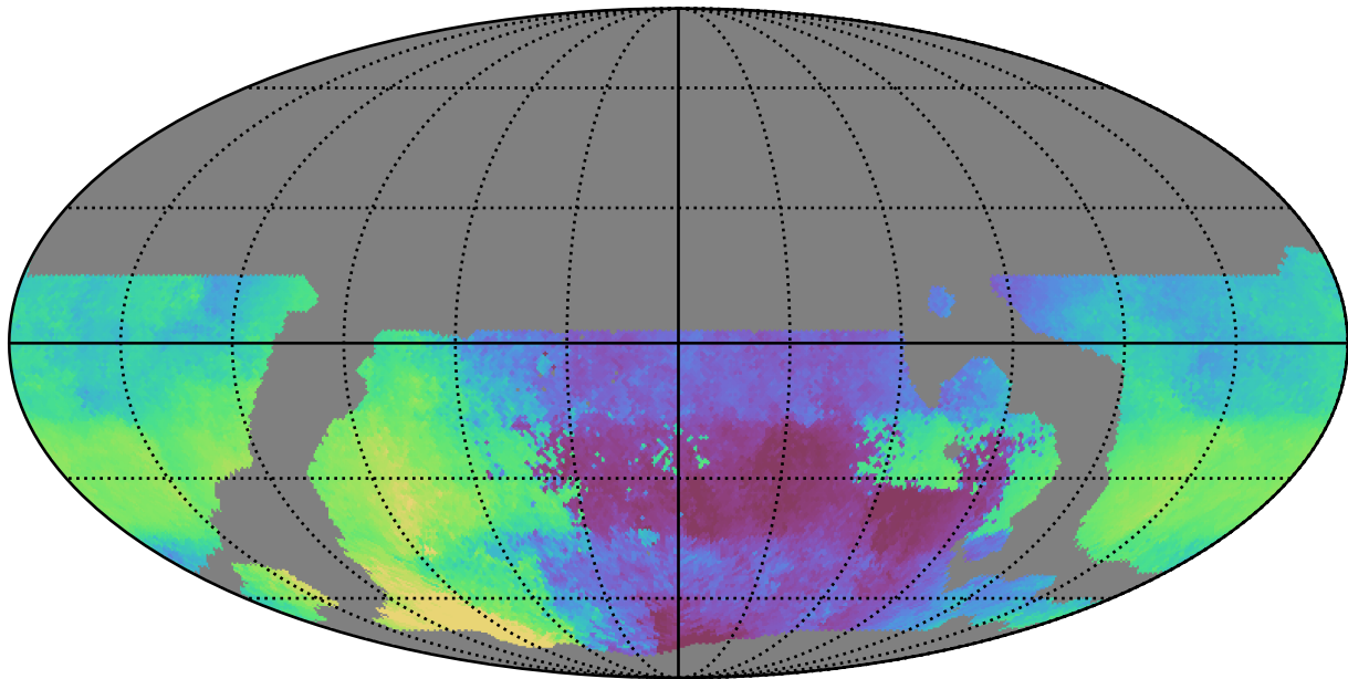
weather_cloudso36v3.4_10yrs WFD u band: Median HA
