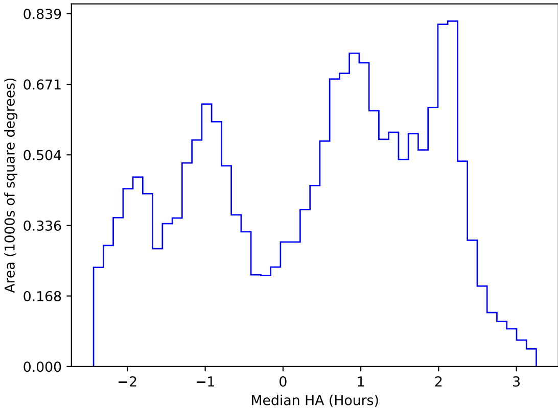
weather_cloudso36v3.4_10yrs WFD u band: Median HA
