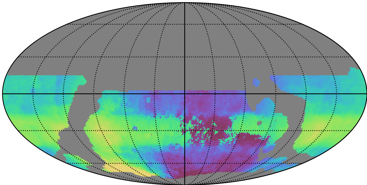
weather_cloudso36v3.4_10yrs WFD r band: Median HA
