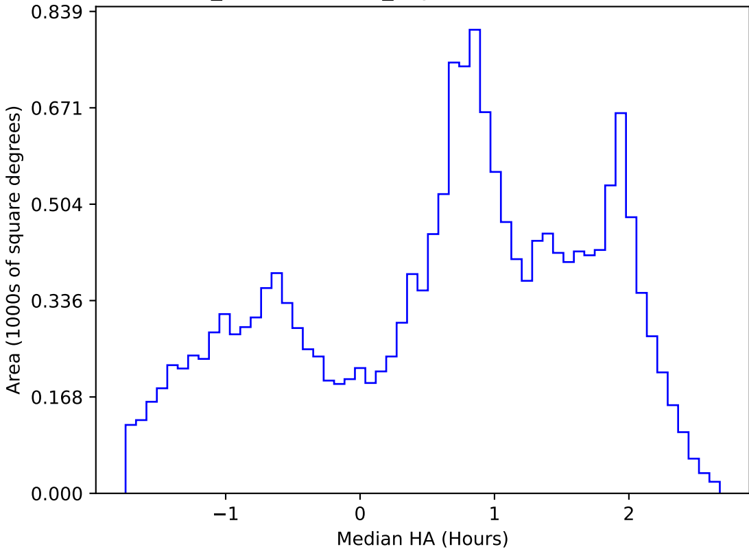
weather_cloudso36v3.4_10yrs WFD r band: Median HA
