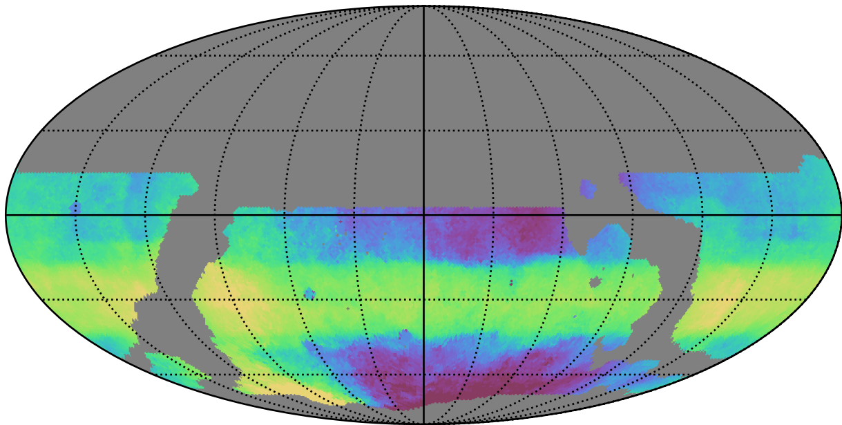
weather_cloudso36v3.4_10yrs WFD i band: Median HA
