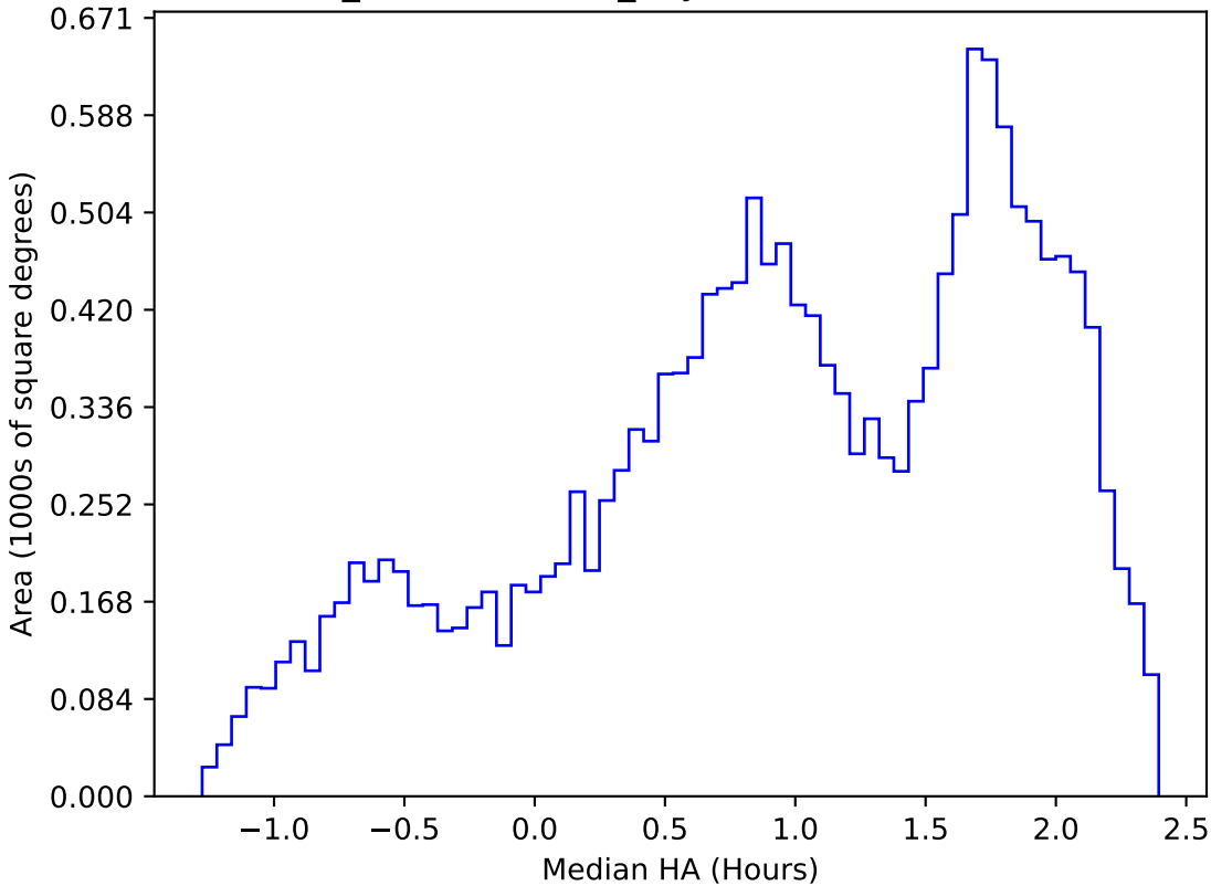
weather_cloudso36v3.4_10yrs WFD i band: Median HA
