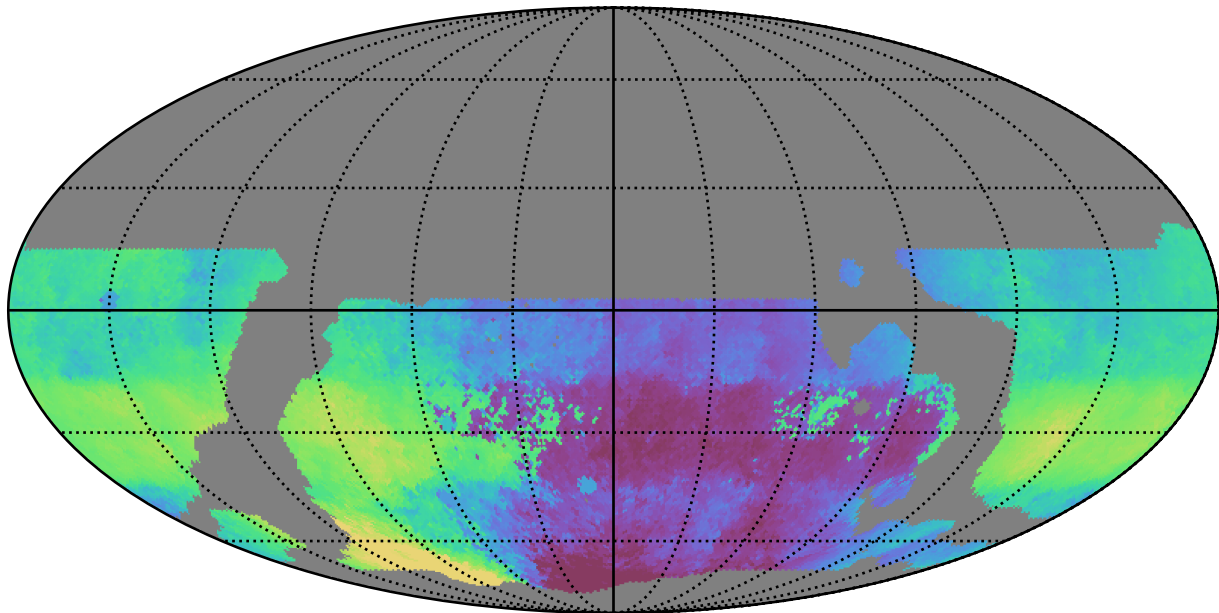
weather_cloudso36v3.4_10yrs WFD g band: Median HA
