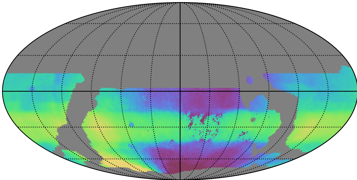
weather_cloudso36v3.4_10yrs WFD all bands: Median HA
