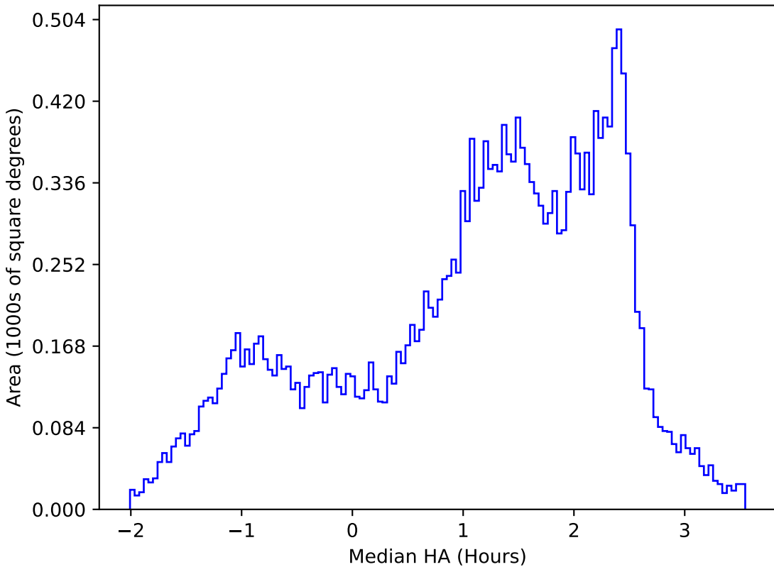
weather_cloudso36v3.4_10yrs All sky y band: Median HA
