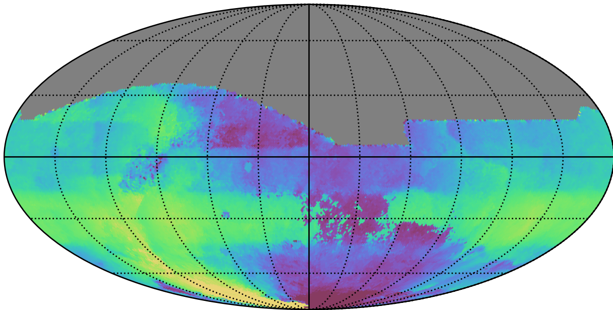
weather_cloudso36v3.4_10yrs All sky r band: Median HA
