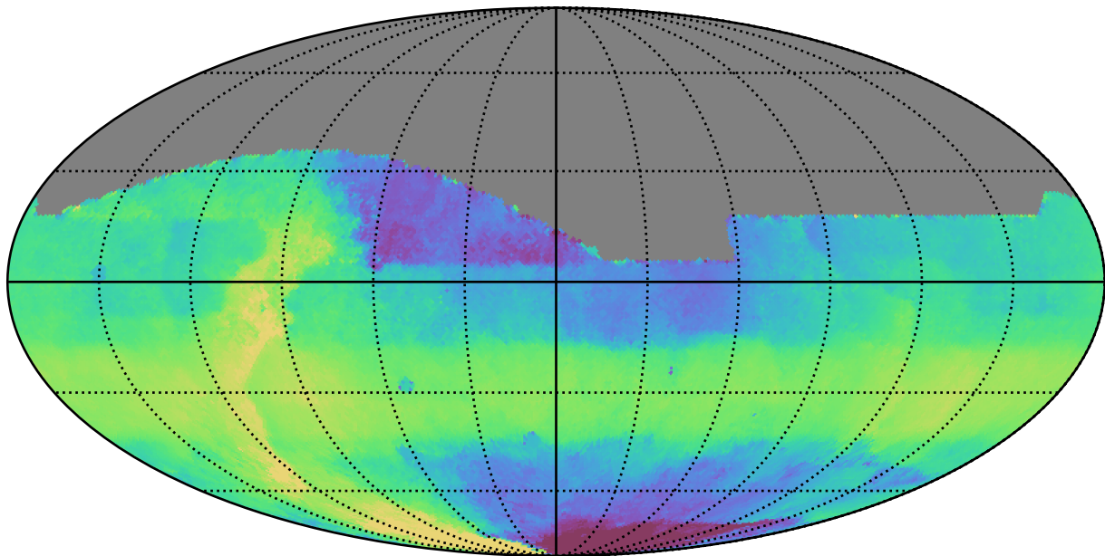
weather_cloudso36v3.4_10yrs All sky i band: Median HA
